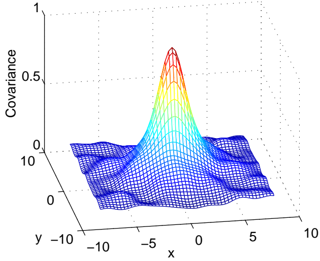
Covariance B(z)
