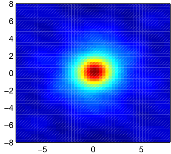
Intensity plot of covariance
