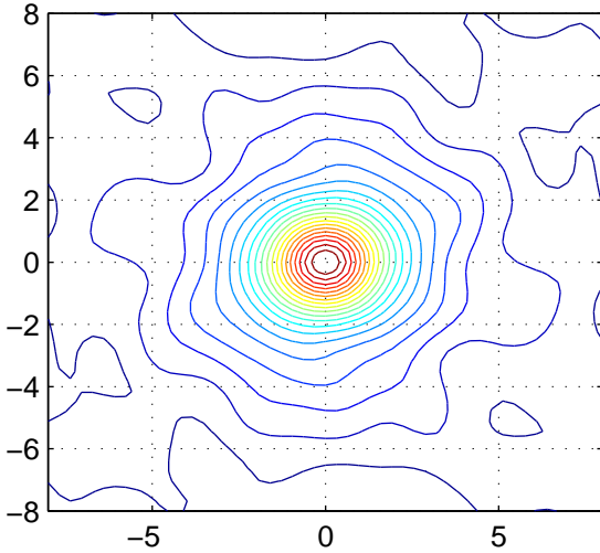
Contour plot of covariance
