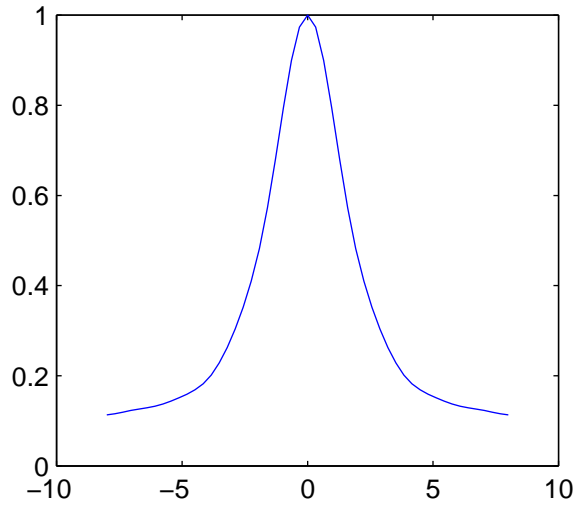
Covariance in the x direction
