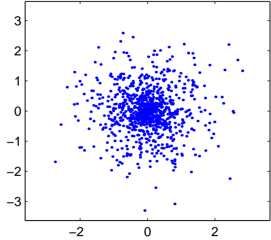
Wavenumbers K
