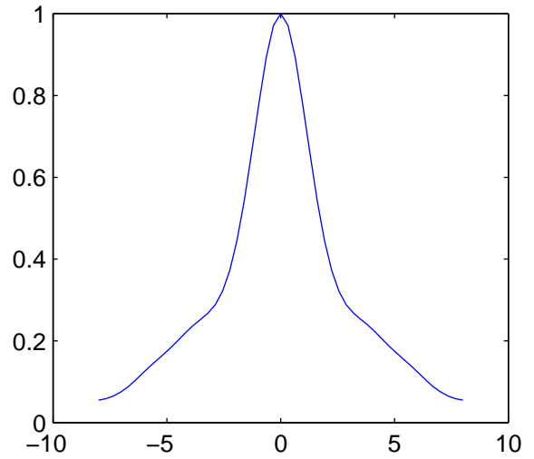
Covariance in the y direction
