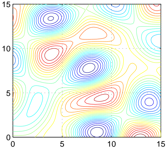
Contour plot
