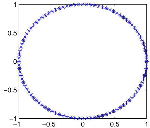
Wavenumbers K
