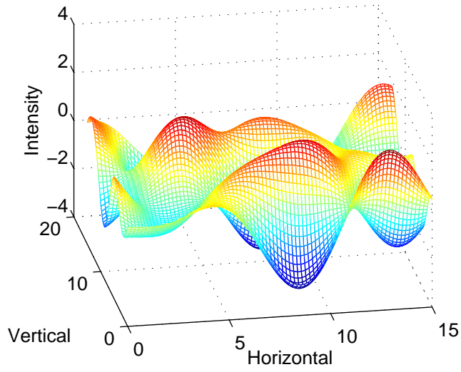
Surface plot
