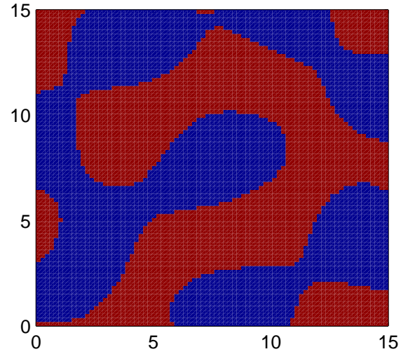
Level sets
