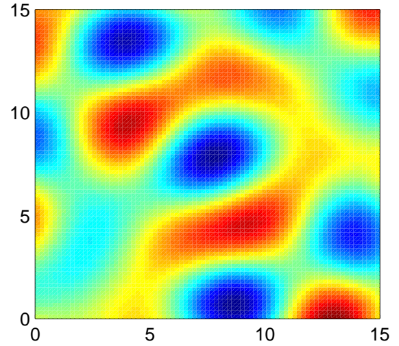
Intensity plot
