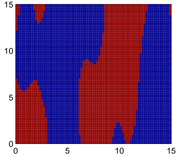
Level sets
