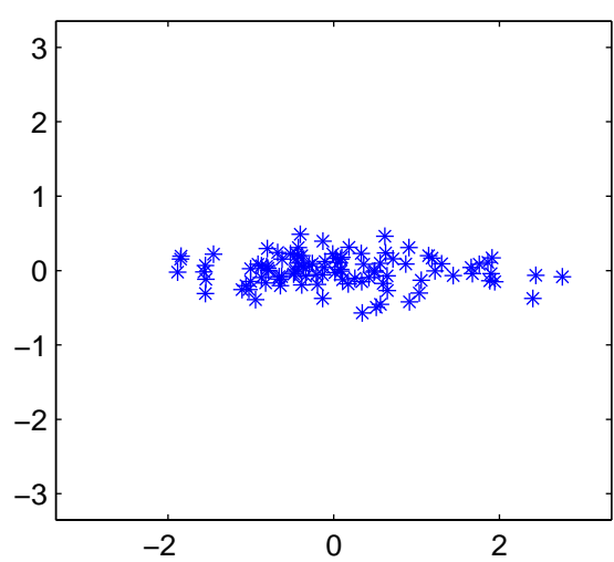
Wavenumbers K
