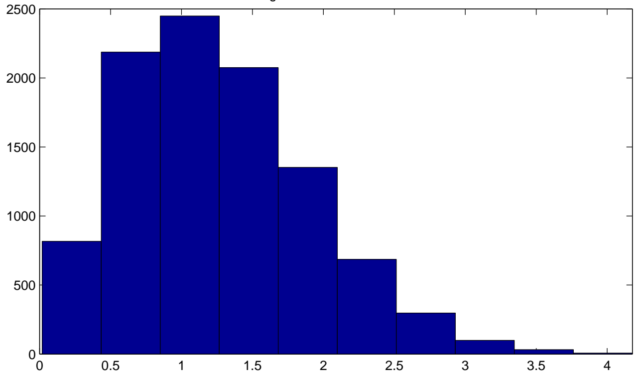
Histogram of wavenumber norms
