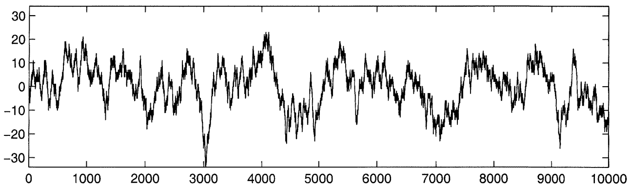
Ornstein-Uhlenbeck process
