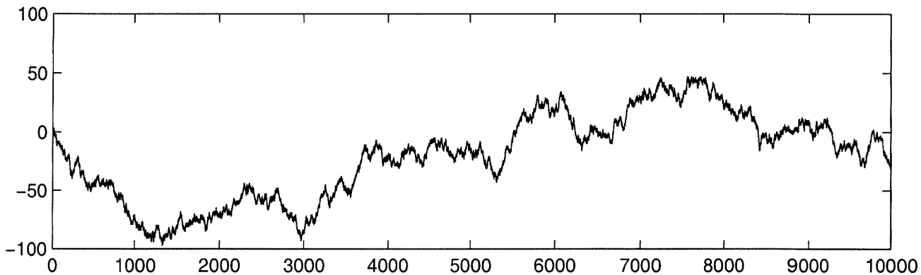
Ehrenfest urn model
