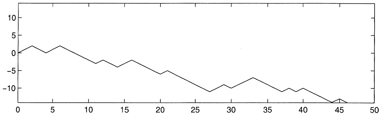
Brownian motion
